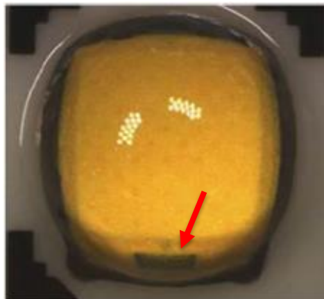
LUXEON TX with current TVS chip
