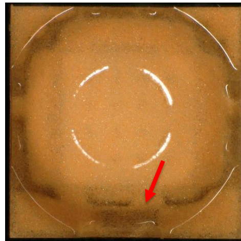
LUXEON C with alternate TVS chip
