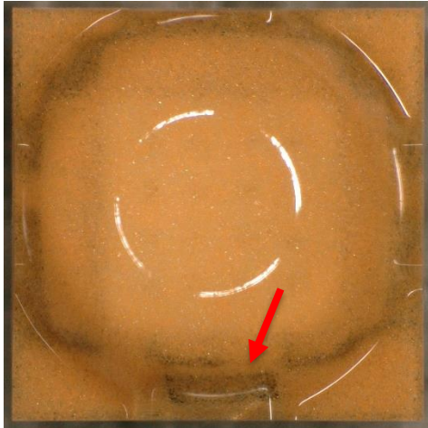
LUXEON C with current TVS chip
