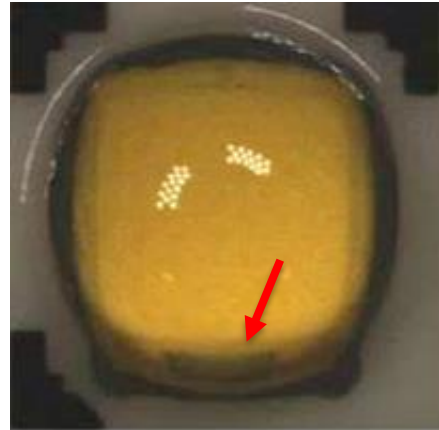
LUXEON TX with alternate TVS chip
