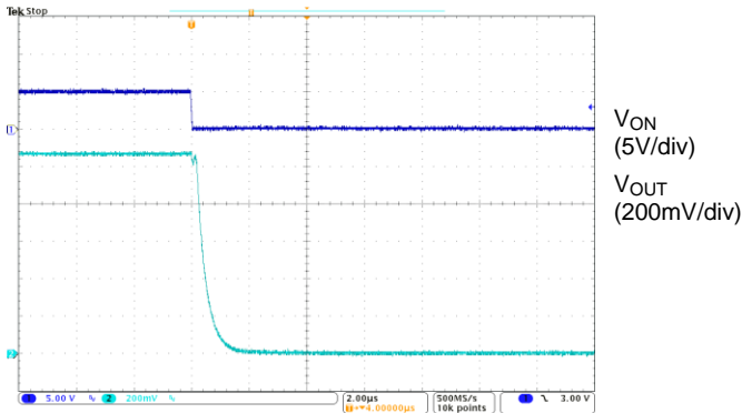
Turn-OFF & Turn-OFF Fall Times V_{IN} = 1.05\text{V} , V_{VBIAS} = 5\text{V} , C_{IN} = 1\mu\text{F} , C_{OUT} = 0.1\mu\text{F} , R_{OUT} = 10\Omega
