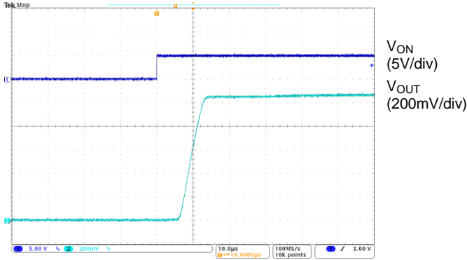
Turn-ON & Turn-ON Rise Times V_{IN} = 1.05\text{V} , V_{VBIAS} = 5\text{V} , C_{IN} = 1\mu\text{F} , C_{OUT} = 0.1\mu\text{F} , R_{OUT} = 10\Omega
