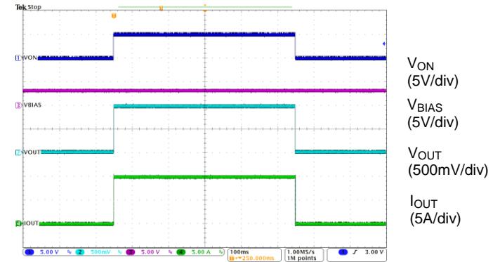
Turn-ON & Turn-OFF at I_{OUT} = -10\text{A} V_{IN} = 1.05\text{V} , V_{VBIAS} = 3.2\text{V} , C_{IN} = 1\mu\text{F} , C_{OUT} = 0.1\mu\text{F} , R_{OUT} = 0.1\Omega
