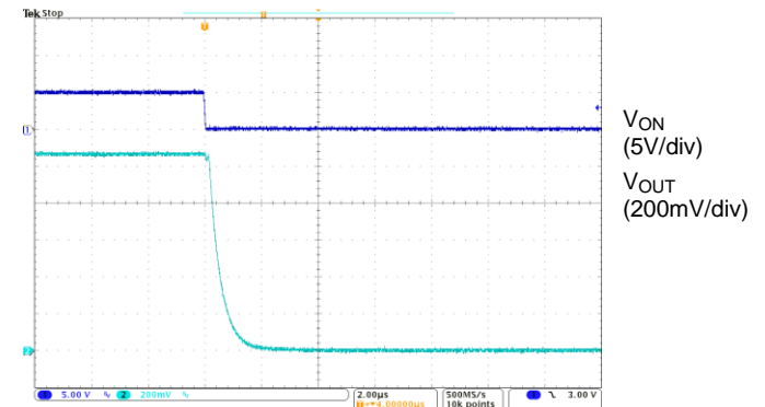
Turn-OFF & Turn-OFF Fall Times V_{IN} = 1.05\text{V} , V_{VBIAS} = 3.2\text{V} , C_{IN} = 1\mu\text{F} , C_{OUT} = 0.1\mu\text{F} , R_{OUT} = 10\Omega
