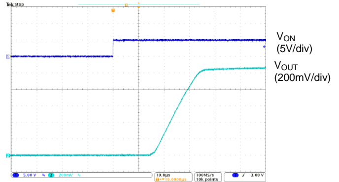
Turn-ON & Turn-ON Rise Times V_{IN} = 1.05\text{V} , V_{VBIAS} = 3.2\text{V} , C_{IN} = 1\mu\text{F} , C_{OUT} = 0.1\mu\text{F} , R_{OUT} = 10\Omega
