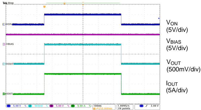
Turn-ON & Turn-OFF at I_{OUT} = -10\text{A} V_{IN} = 1.05\text{V} , V_{VBIAS} = 5\text{V} , C_{IN} = 1\mu\text{F} , C_{OUT} = 0.1\mu\text{F} , R_{OUT} = 0.1\Omega
