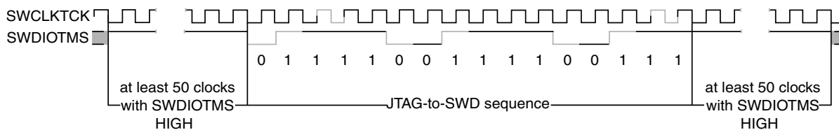
Figure 9-28. JTAG-to-SWD switching sequence
