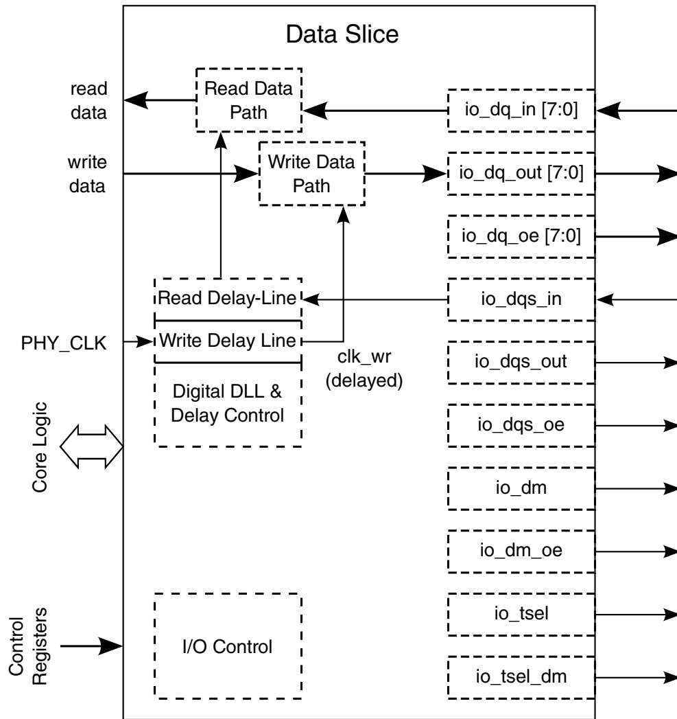
Figure 10-9. DDR PHY Data Slice
