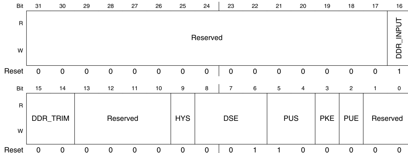
IOMUXC_DDR_A_12 field descriptions
