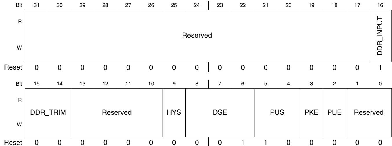
IOMUXC_DDR_BA_1 field descriptions
