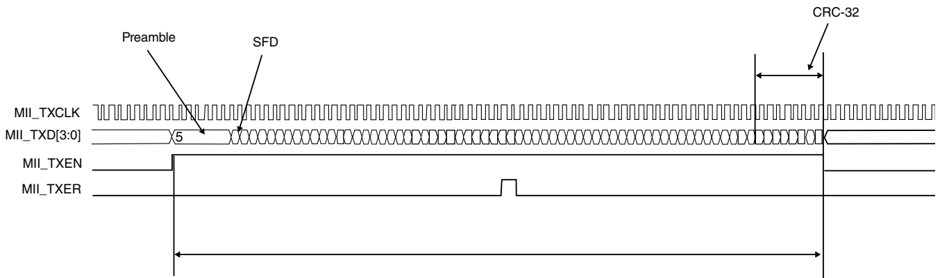
Figure 11-56. MII transmit operation — errored frame
