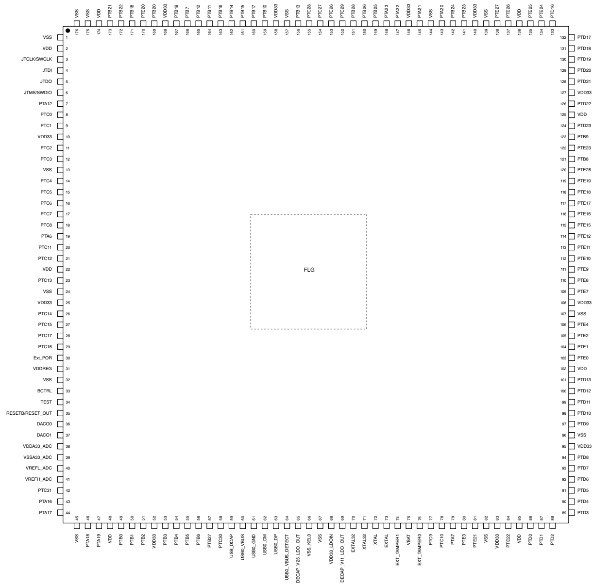
Figure 5-1. 176 LQFP Pinout Diagram
