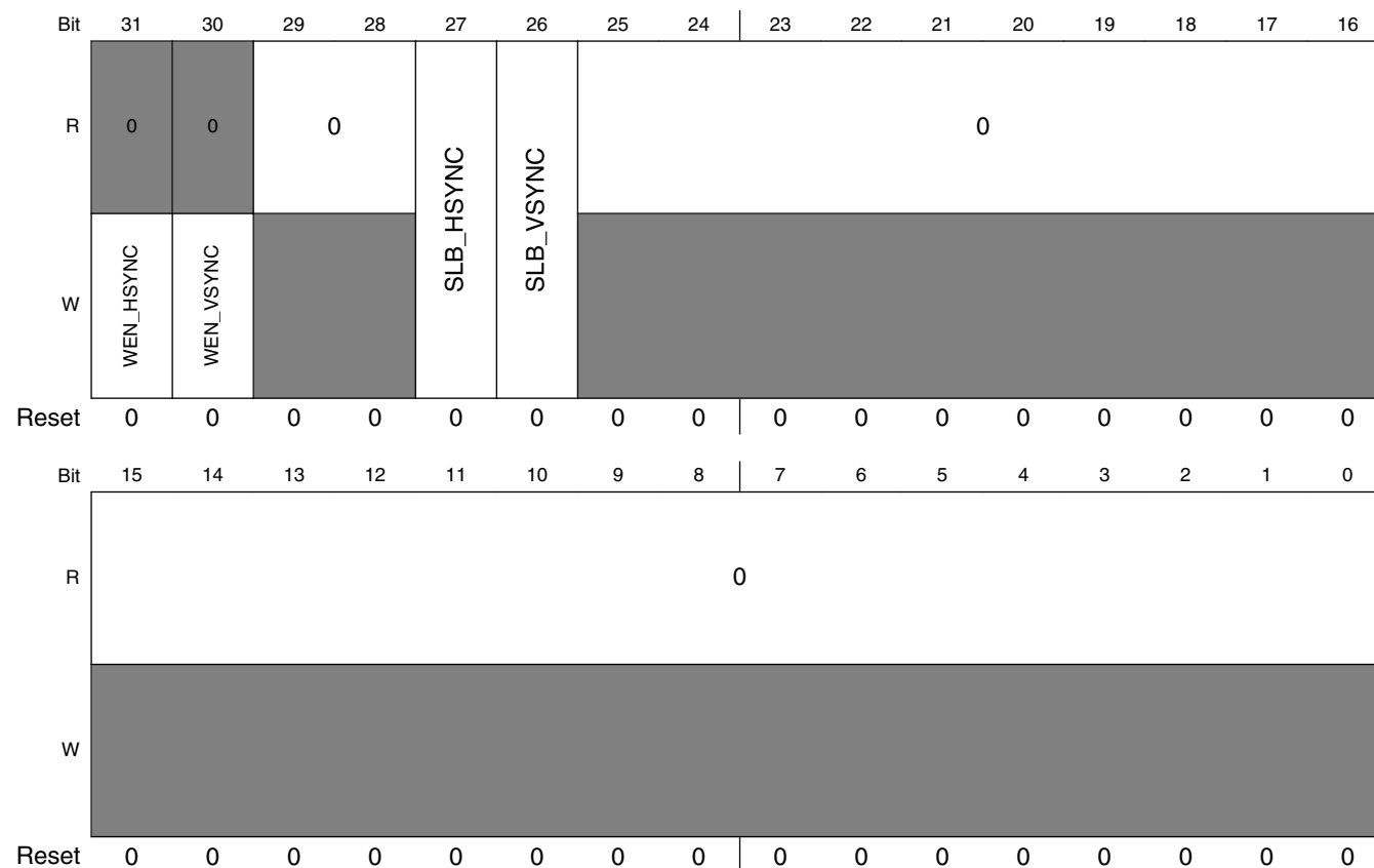
DCUx_SFT_LCK_HS_VS_PARA field descriptions
