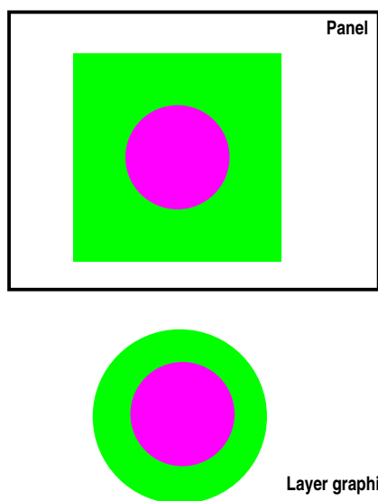
Figure 16-12. Case 9 example (no blend, pixel alpha ignored)
