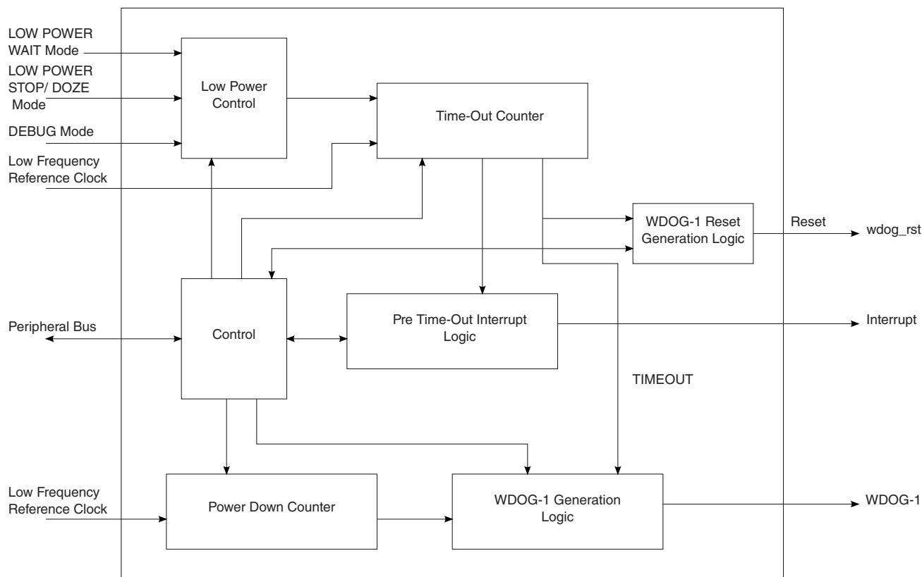
Figure 9-15. WDOG Diagram
