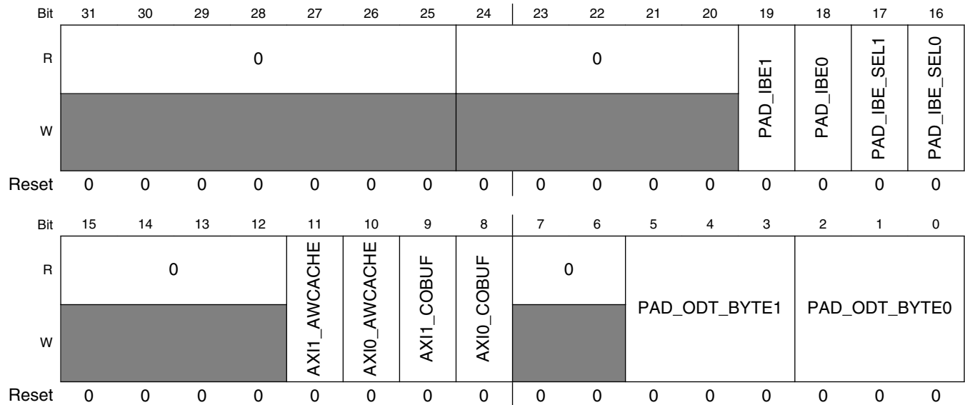
DDRMC_CR155 field descriptions
