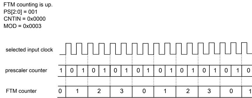
Figure 13-3. Example of the prescaler counter
