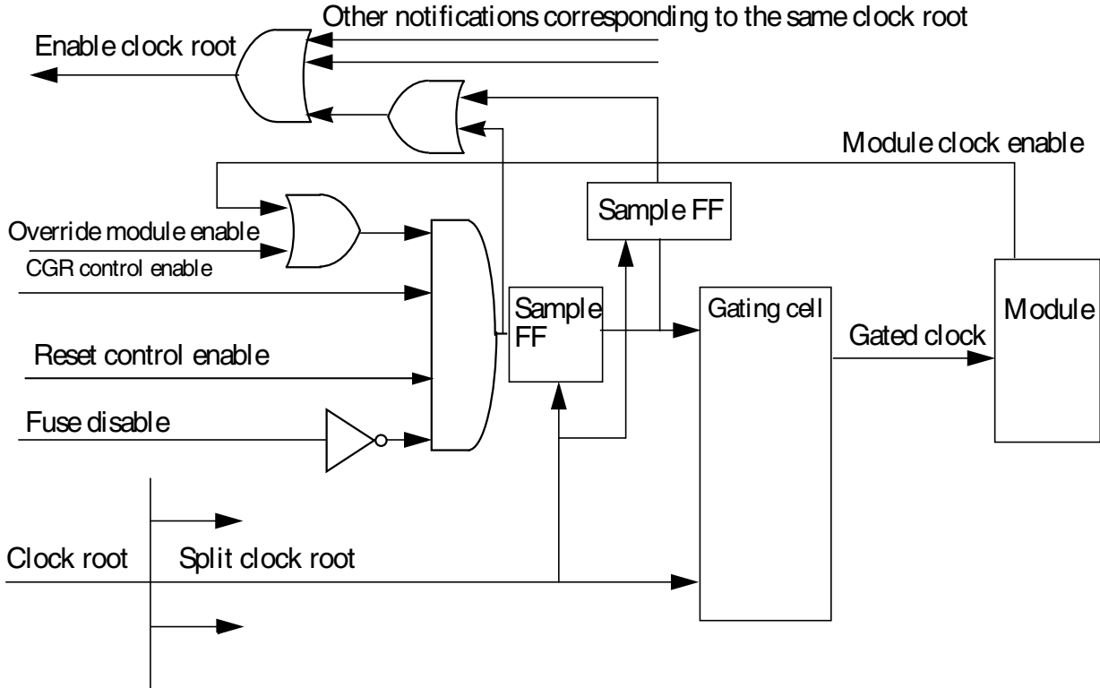
Figure 6-20. Implementation for each gating cell
