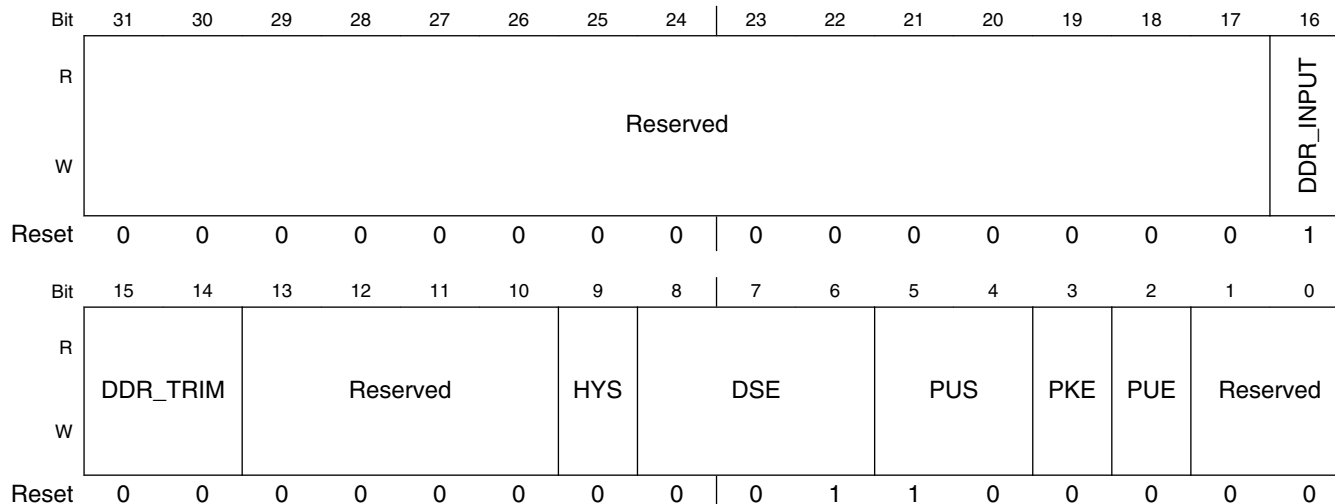
IOMUXC_DDR_A_4 field descriptions
