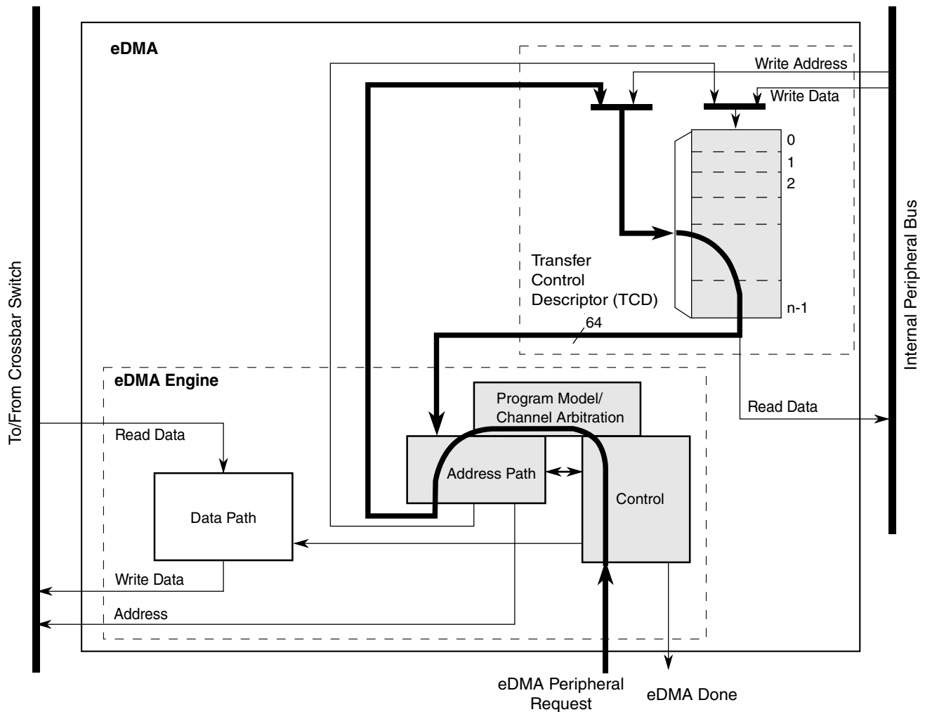
Figure 14-2. eDMA operation, part 1
