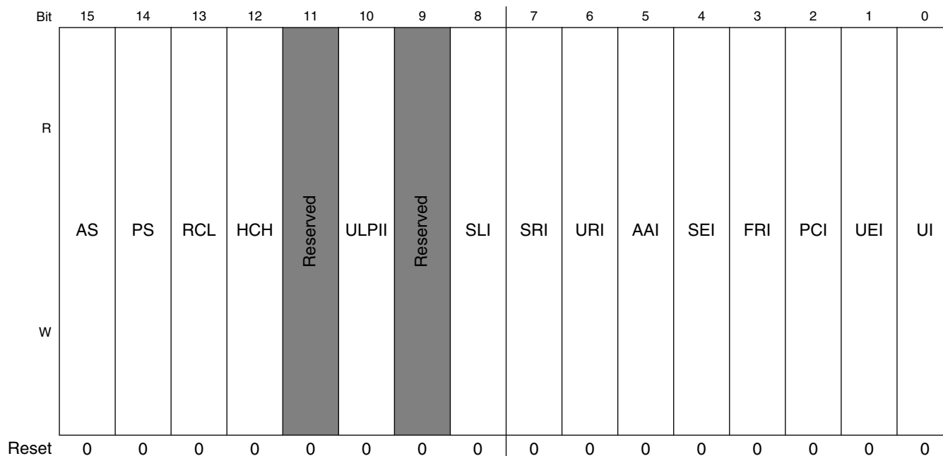
USBx_USBSTS field descriptions
