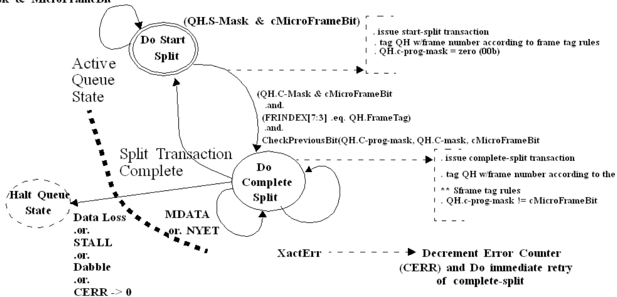
Figure 11-23. Split Transaction State Machine for Interrupt
