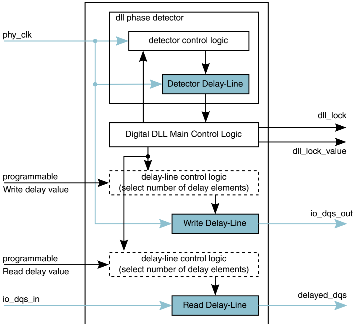
Figure 10-13. Digital DLL
