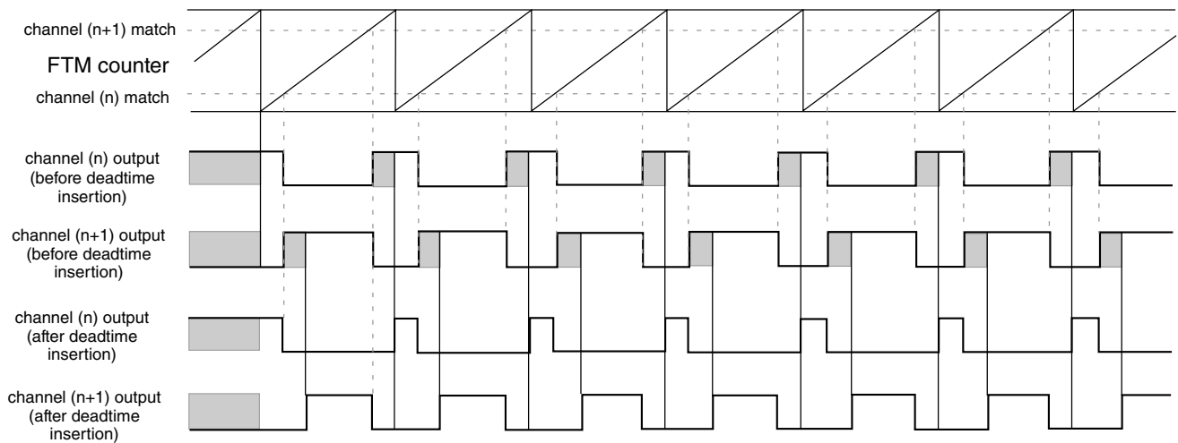
Figure 13-66. Deadtime insertion with ELSnB:ELSnA = X:1, POL(n) = 0, and POL(n+1) = 0
