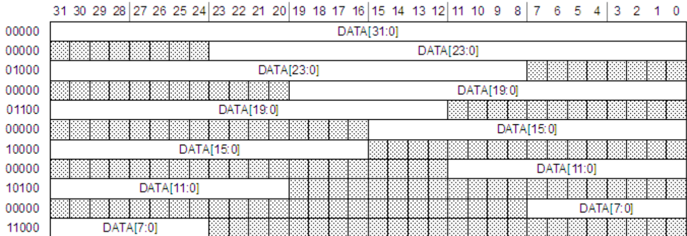
Figure 15-2. SAI first bit shifted, LSB first
