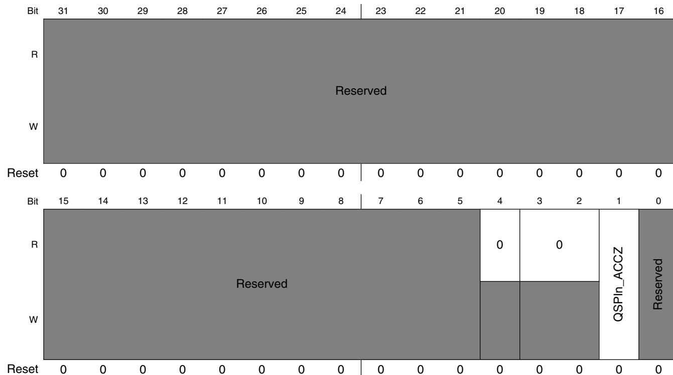
CCM.CGPR field descriptions
