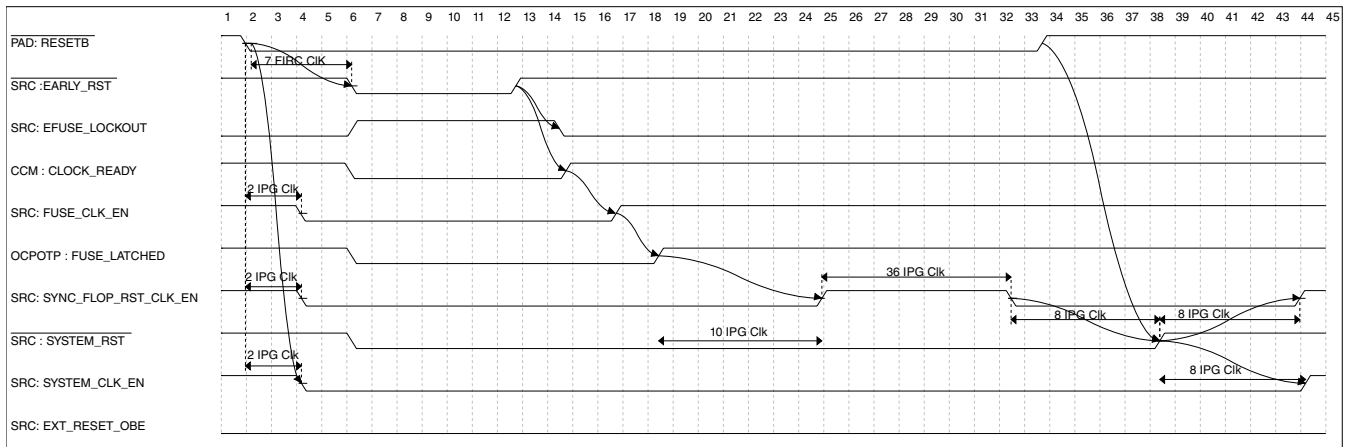
Figure 7-9. External reset sequence
