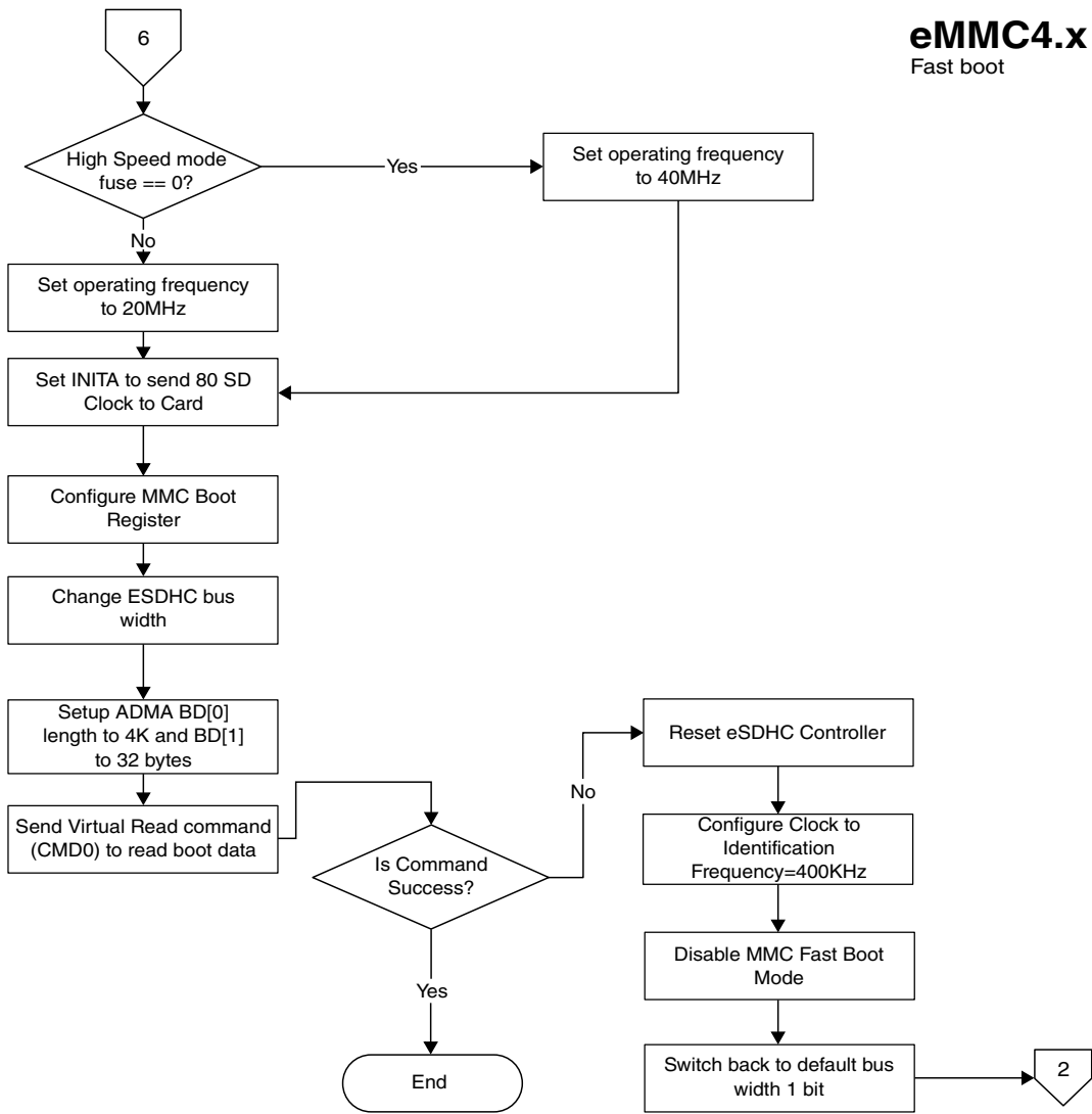
Figure 7-26. Expansion Device Boot Flow (2/7)
