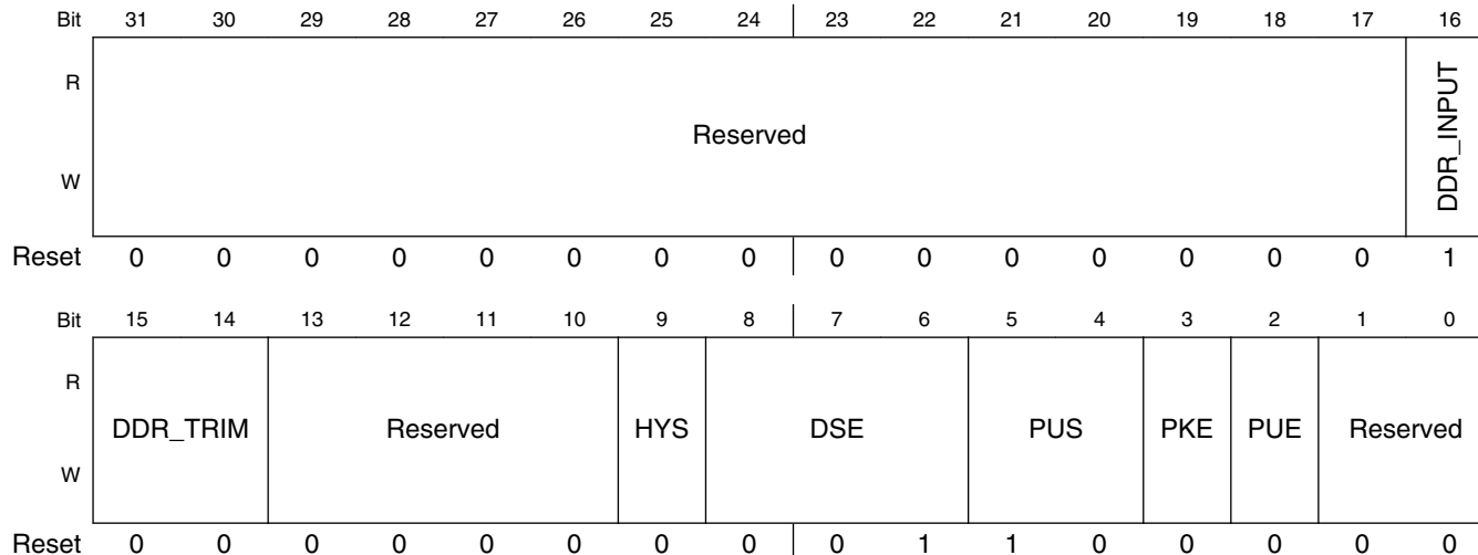
IOMUXC_DDR_DQM_1 field descriptions
