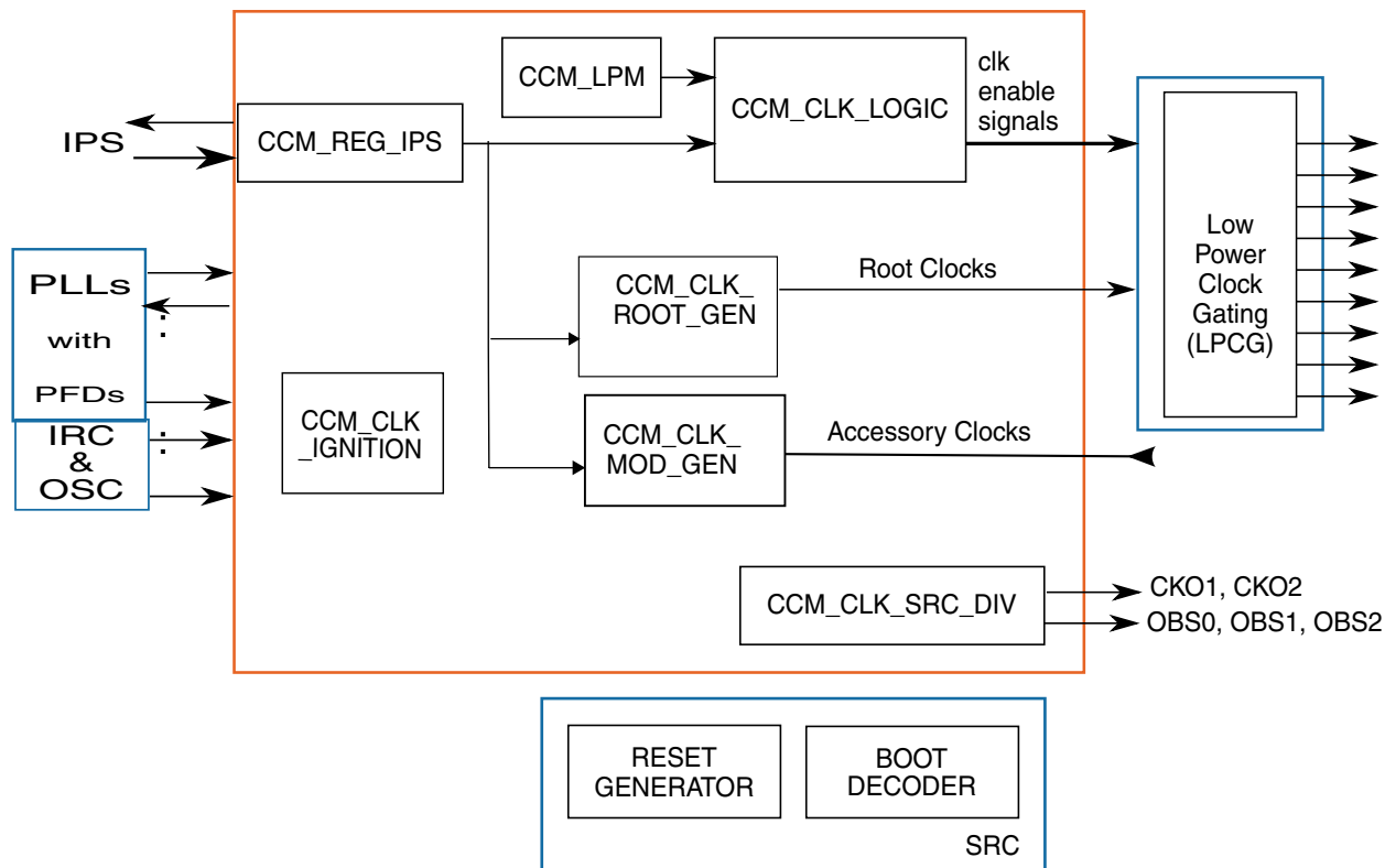
Figure 6-18. Block Diagram
