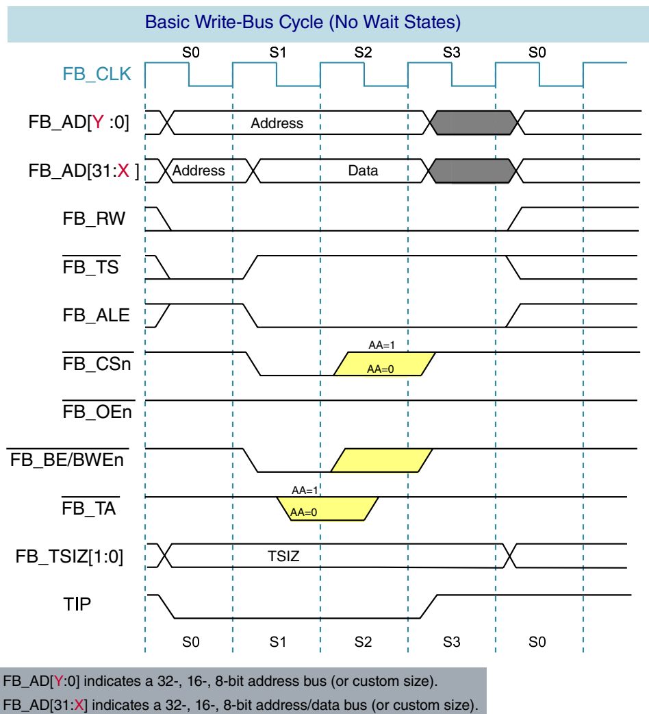
Figure 10-68. Basic Write-Bus Cycle (No Wait States)
