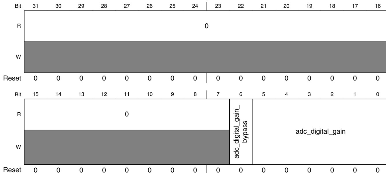
AFE_ADCDGN field descriptions
