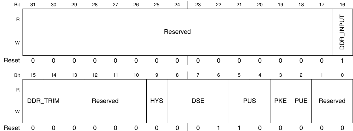
IOMUXC_DDR_A_14 field descriptions
