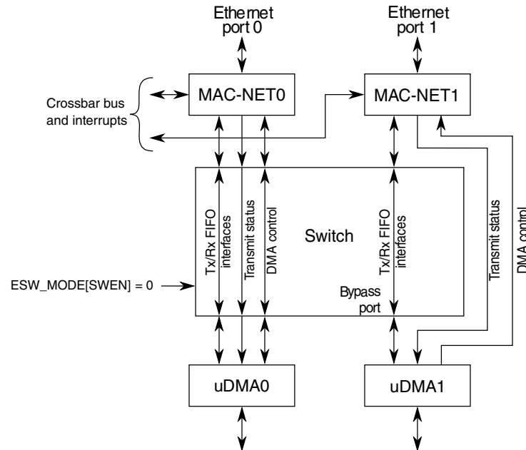
Figure 11-61. Passthrough Mode Configuration Overview
