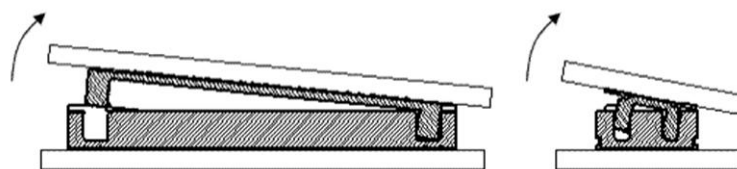
× 図-5 こじり抜去 (Not Good) Figure-5 Withdrawal with twisting the connector at an angle (Not Good)
